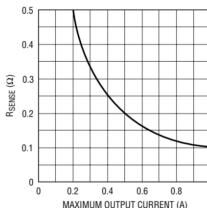
Figure 2. Selecting R_{\text{SENSE}}
