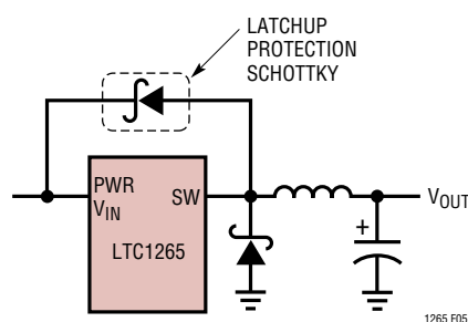
Figure 5. Preventing Absolute Maximum Ratings from Being Exceeded
